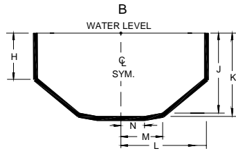
CROSS SECTION AT POINT B
