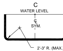
CROSS SECTION AT POINT C
