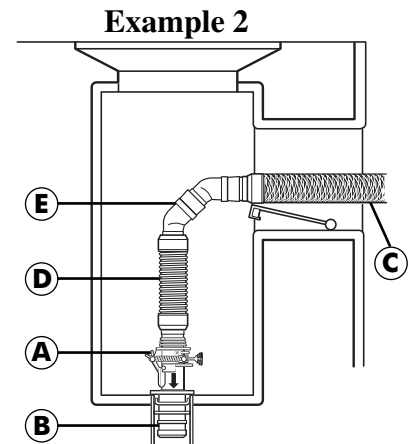
(1) 4 1/2" Connector
